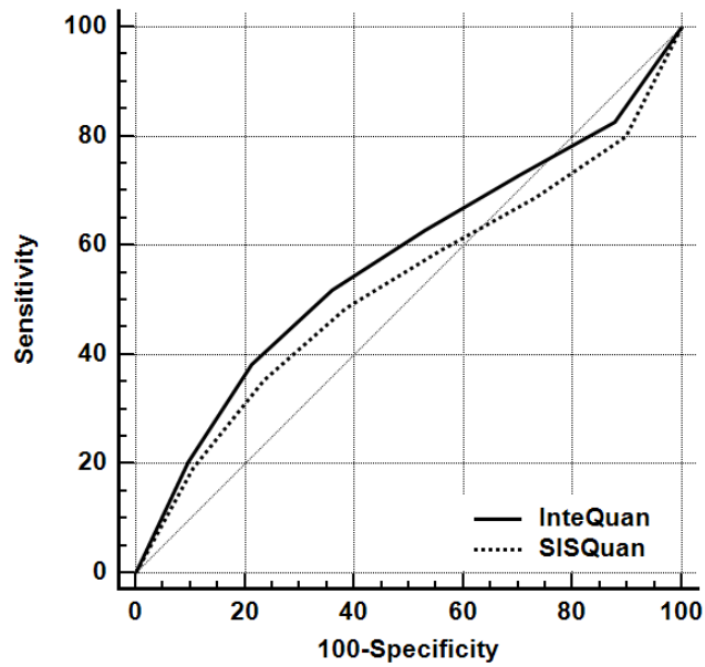
Figure S2 Receiver operating characteristic curves of the panel of all 16 target proteins, evaluated with Monte Carlo cross validation (MCCV) on clinical samples in Study I. Proteins were quantified using InteQuan (solid line) or SISQuan (dotted line).
