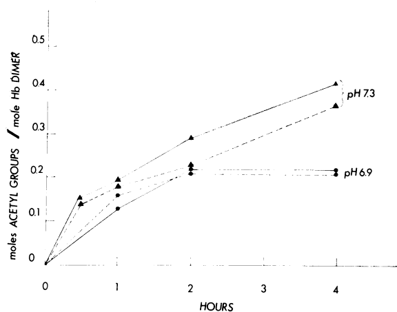
FIGURE 1 Incorporation of ^{14}\text{C} -acetyl groups into hemoglobin. Red cells were incubated with 20 mM [ acetyl-1- ^{14}\text{C} ]ASA in isotonic phosphate buffer, pH 7.3 ( \blacktriangle ) and pH 6.9 ( \bullet ), at 37^\circ\text{C} for 4 h. The acetylation of hemoglobin was estimated from radioactivity measurements (—) and gel scanning (---).
