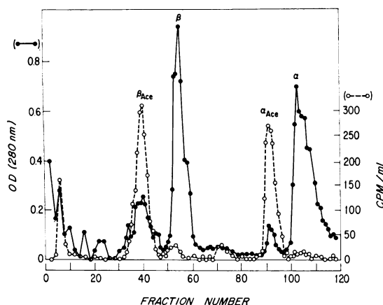
FIGURE 8 Separation of acetylated and nonacetylated globin subunits by chromatography on CM-cellulose in 8 M urea. Purified human hemoglobin A was incubated for 20 h with 2.0 mM [ acetyl -1- 14 C]ASA in 0.1 M phosphate buffer, pH 7.3, 37°C.
