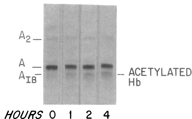
FIGURE 2 Separation of acetylated hemoglobin from normal hemoglobin A by isoelectric focusing on polyacrylamide gel. Red cells were incubated with 20 mM ASA in isotonic phosphate buffer, pH 6.9, at 37^\circ\text{C} for 4 h. The results of quantitative scanning of these gels are shown in Fig. 1.
