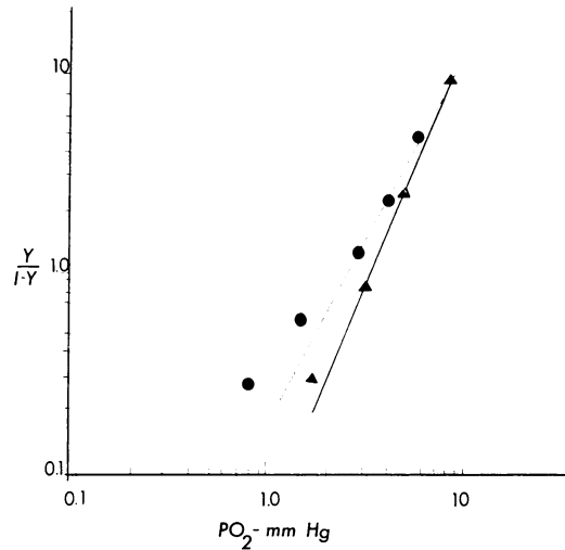
FIGURE 4 Oxygen equilibria on acetylated (●) and non-acetylated (▲) hemoglobins isolated by column chromatography (see Fig. 3). 0.1 mM hemoglobin tetramer in 0.1 M \text{Cl}^- , 0.05 M bis-Tris, pH 7.2, 20°C.
