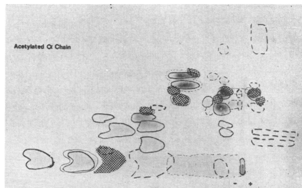
FIGURE 9 Fingerprint of 14 C-acetylated \alpha -chains. After cellulose thin layer plate was stained with ninhydrin, the positive spots were circled. The plate was then autoradiographed for 15 days. The radioactive spots are indicated by stippled areas.
