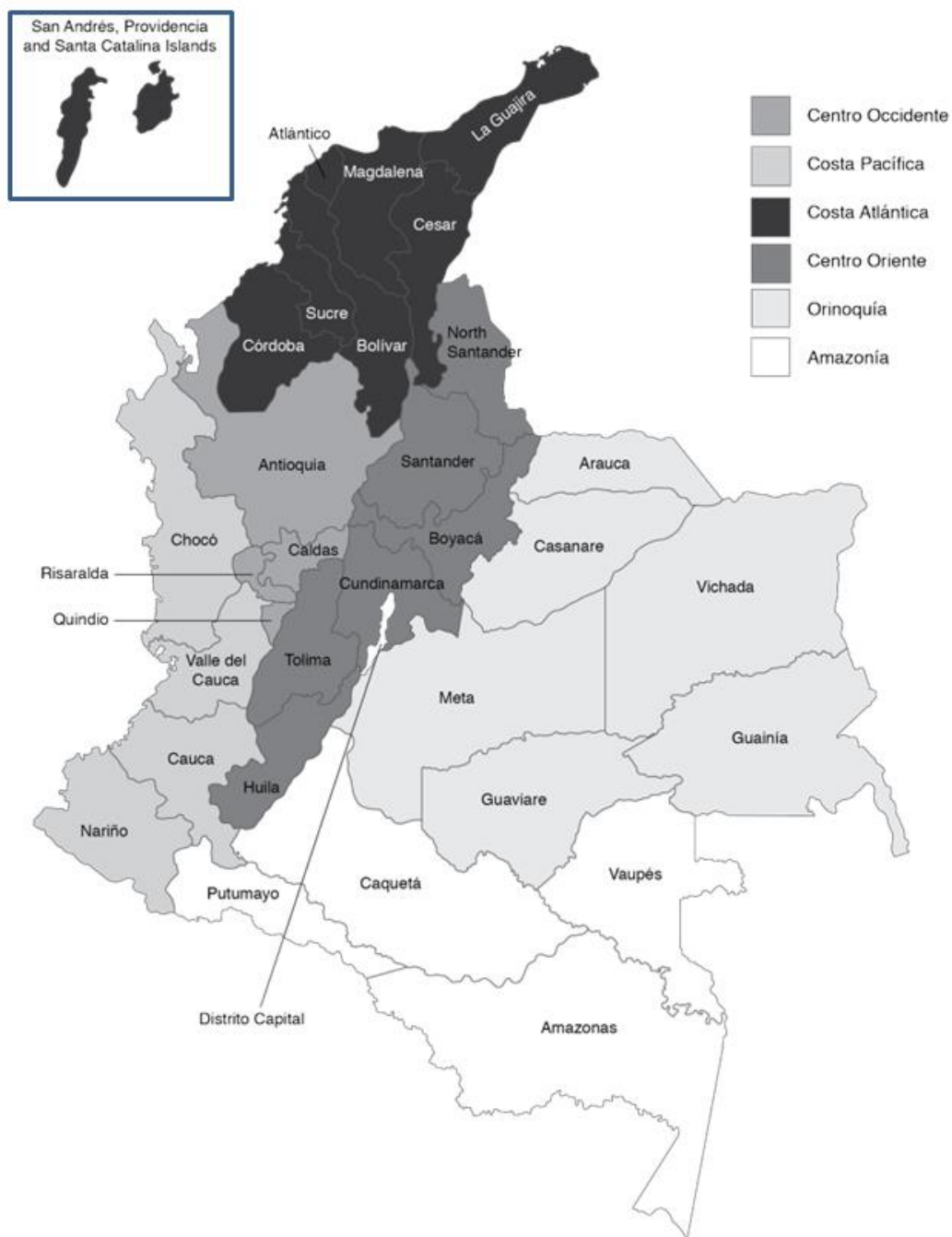
Figure S1. Departments of Colombia.
