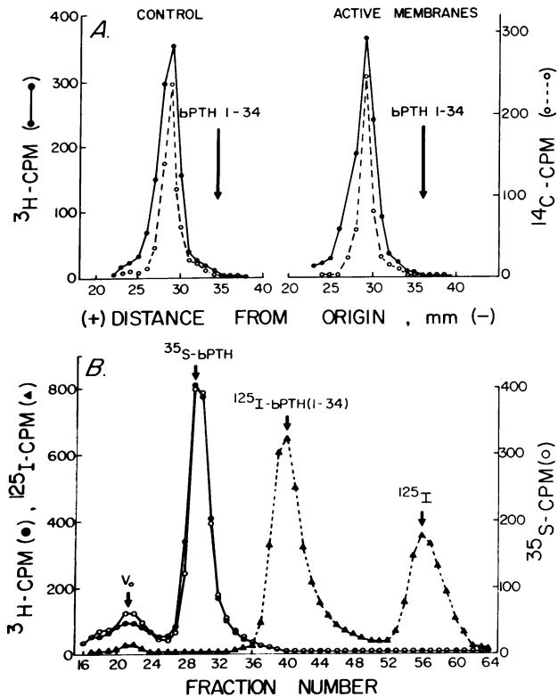
FIGURE 2 Analysis of [ ^3\text{H} ]bPTH-(1-84), after incubation with canine renal cortical membranes for 10 min at 22°C, by electrophoresis (Fig. 2A) on polyacrylamide gels at pH 4.4, and by chromatography (Fig. 2B) on Bio-Gel A-0.5m with 6 M guanidine HCl-0.1 M ammonium acetate-1% (vol/vol) human plasma, pH 6.5, as eluting buffer. For electrophoresis (Fig. 2A), [ ^{14}\text{C} ]bPTH-(1-84) was added to the gels to serve as an internal marker for intact hormone. The arrow (Fig. 2A) represents the migration position of ^{125}\text{I} -labeled bPTH-(1-34) run in parallel gels. "Control" (Fig. 2A) represents the pattern obtained after incubation of [ ^3\text{H} ]bPTH-(1-84) with heat-inactivated membranes. For chromatography (Fig. 2B), [ ^{35}\text{S} ]bPTH-(1-84) was added to the column to serve as an internal marker for intact hormone. The column was subsequently calibrated with ^{125}\text{I} -labeled bPTH-(1-34) and \text{Na}^{125}\text{I} to mark the elution positions of active fragment and salt peak, respectively. V_0 represents the void volume. A pattern of radioactivity identical with Fig. 2B was obtained after incubation of [ ^3\text{H} ]bPTH-(1-84) with heat-inactivated membranes. Details of the incubation, electrophoresis, and chromatography are described in the text.
