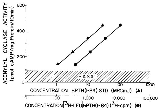
FIGURE 1 Dose-response curve of [ 3 H]bPTH-(1–84) (●—●) in canine renal cortical membranes. Unlabeled bPTH-(1–84) (▲—▲) (MRC Research Standard 72/286) was used as a standard. Adenylyl cyclase assay was performed at 37°C as described in Methods. Each point represents the mean of duplicate determinations ± SE. “Basal” represents adenylyl cyclase activity in the absence of hormone.
