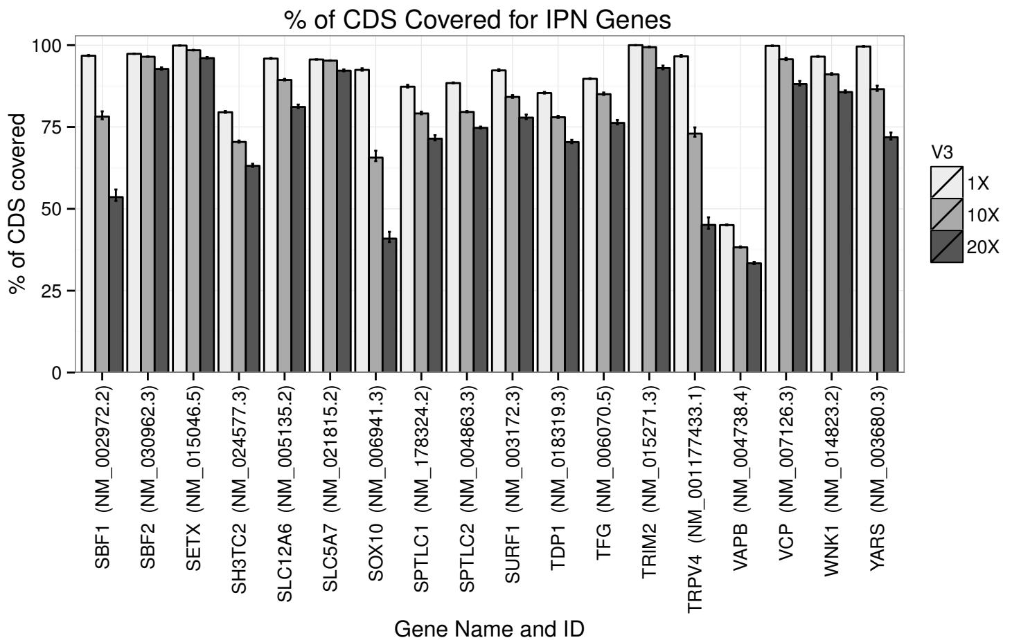
Supplementary Figure S1 C - D: Mean percentage of the CDS covered by WES in 112 samples at defined read-depths of 1X, 10X and 20X. Error bars show 95% confidence interval.
