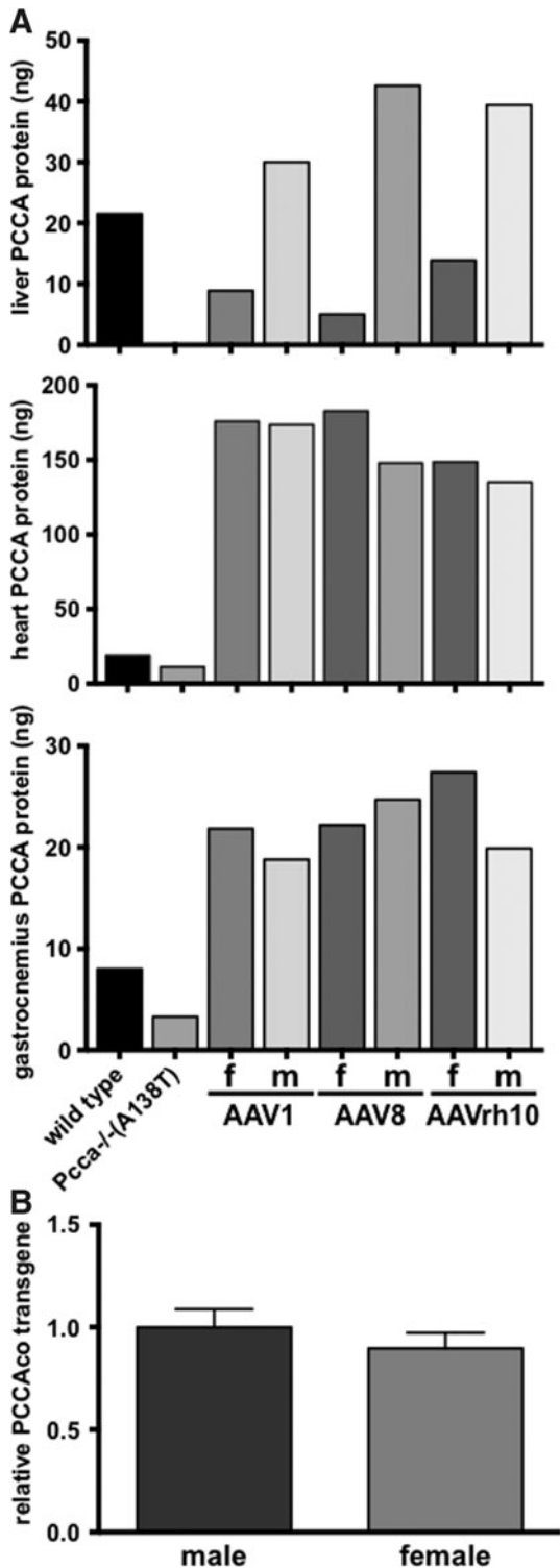
SUPPLEMENTARY FIG. S1. Vector copy analysis. (A) Quantitation of selected Western blot images from Fig. 3 was performed based on 50 ng of a PCCA protein standard. (B) Twenty-five days after IV administration of 5 \times 10^{11} vg of AAV-PCCAcO, livers were removed from male and female Pcca -/- (A138T) mice. DNA was isolated and qPCR specific for PCCAcO transgene and a mouse transferrin receptor (Tfrc) reference gene was performed for data normalization.
