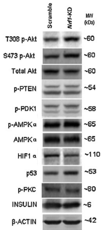
SUPPLEMENTARY FIG. S12. Representative images of immunoblotting of MIN6 cells. n = 2-6 .
