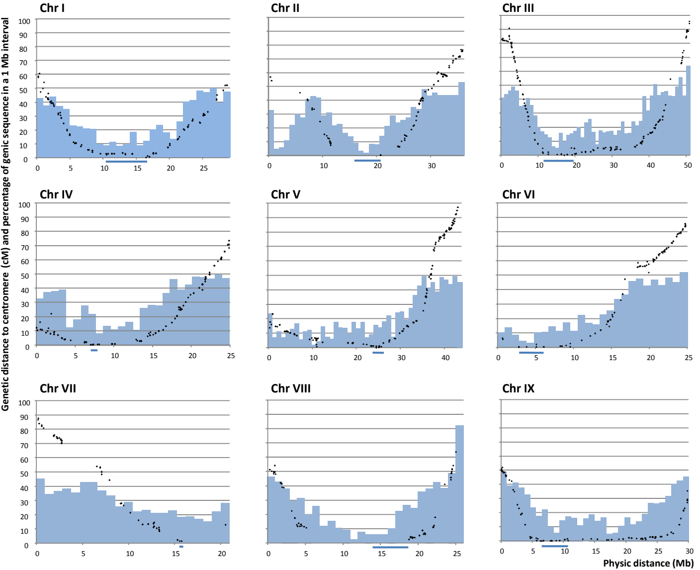
Additional file 9. Relationship between the physical location (x-axis), the genetic distance between centromere and markers on the clementine genetic map (black dots) and the proportion of gene sequences (blue bars) along all chromosomes (Chr). Bars beneath the x-axis indicate the approximate locations of the centromeres location (CI).
