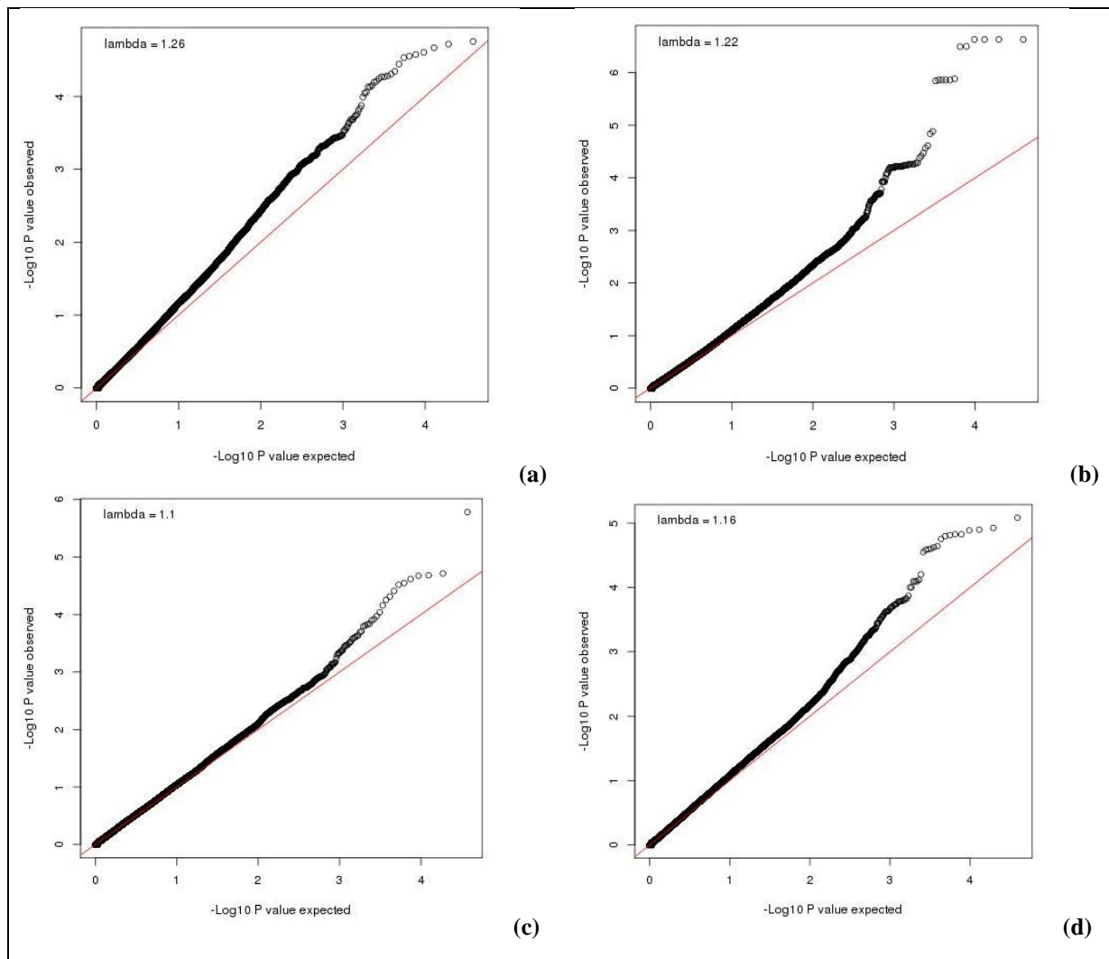
Quantile-quantile plots for cryptorchidism in Large White (a), for cryptorchidism in Landrace (b), for hernia in Large White (c), and for hernia in Landrace (d). Observed distribution of -\log_{10}(\text{P-values}) on the y-axis compared to the expected distribution of -\log_{10}(\text{P-values}) on the x-axis across the 38 632 and 39 508 SNPs for Large White and Landrace, respectively.
