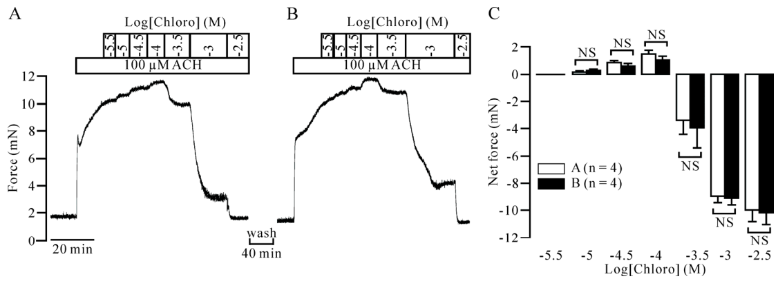
Figure S7. Chloro-induced force changes are reproducible. (A) A typical experiment performed as described in Figure 7A. (B) After washing out chloro and a 40 min rest period, an equivalent experiment was performed. (C) The summarized results. NS: p > 0.05 . These data indicate that chloro can time-independently induce biphasic changes in force.
