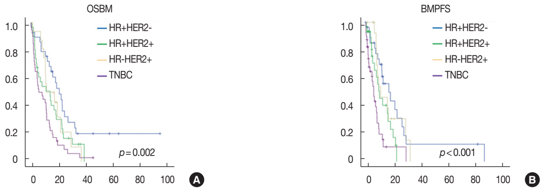
Supplementary Figure 1. Kaplan-Meier plots showing overall survival after brain metastasis (OSBM) and brain metastasis-specific progression-free survival (BMPFS), subdivided by subtypes. All p -values were obtained by the log-rank test. (A) OSBM, p=0.002 . (B) BMPFS, p < 0.001 . HR = hormone receptor; HER2 = human epidermal growth factor receptor 2; TNBC = triple-negative breast cancer.
