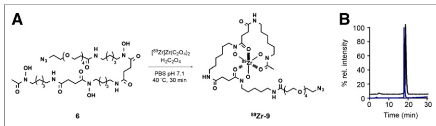
SUPPLEMENTAL FIGURE 3. (A) Radiosynthesis of ^{89}\text{Zr} -9. (B) HPLC chromatogram showing ultraviolet (absorption at 220 nm, front) and radioactive (back) traces of mixture of ^{89}\text{Zr} -9 and reference compound 9, demonstrating coelution.
