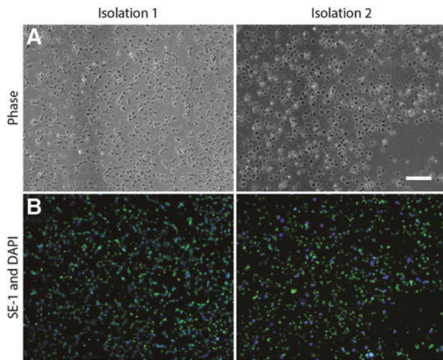
SUPPLEMENTARY FIG. S3. Sinusoidal endothelial 1 (SE-1) stain of liver sinusoidal endothelial cells (LSECs) from both isolations used in a single experiment to make coculture configurations. (A) Phase Images and (B) SE-1 immunostaining LSECs in sandwich culture from different isolations (Day 3) showing similar expression. Scale bar is 100 \mu\text{m} .
