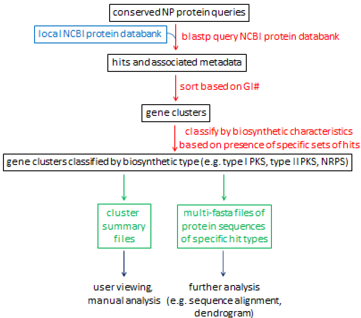
Figure S1. Schematic summary of Dynamite workflow used in this study.
