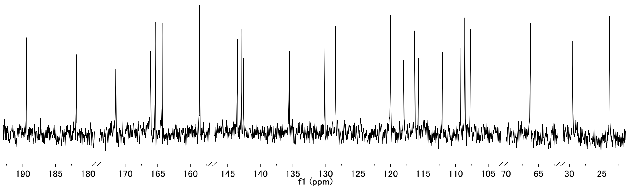
Non-labeled Frankiamicin A, ^{13}\text{C} NMR 75 MHz DMSO- \text{d}_6
