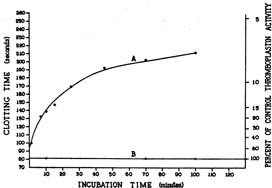
FIG. 4. THE CLOTTING TIMES PRODUCED BY BARIUM SULFATE-ADSORBED SERUM, DILUTED THROMBOPLASTIN AND CALCIUM CHLORIDE INCUBATED TOGETHER AT 37° C. AND ADDED TO A CLOTTING SYSTEM AT INTERVALS
