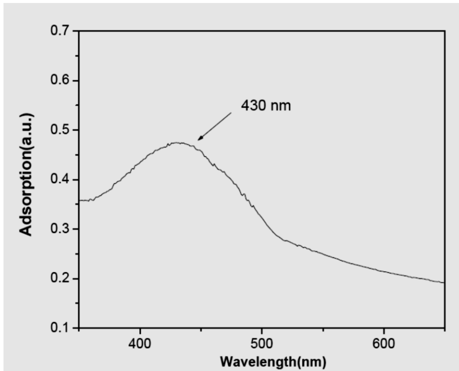
Figure S1. UV-vis absorption of Ag NPs with 22 nm in diameter deposited on PDMS through a photo-reduction process.
