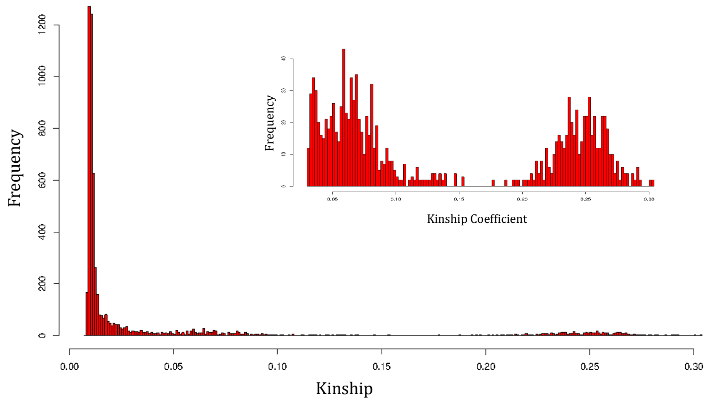
Histogram showing the distribution of pairwise kinship coefficients (smaller picture is zoomed into the part of the graph in which the coefficient is greater than 0.03125, n=1593 ). The peak over 0.25 represents siblings. The peak close to 0.25 second degree relatives and at 0.0625 third degree relatives.
