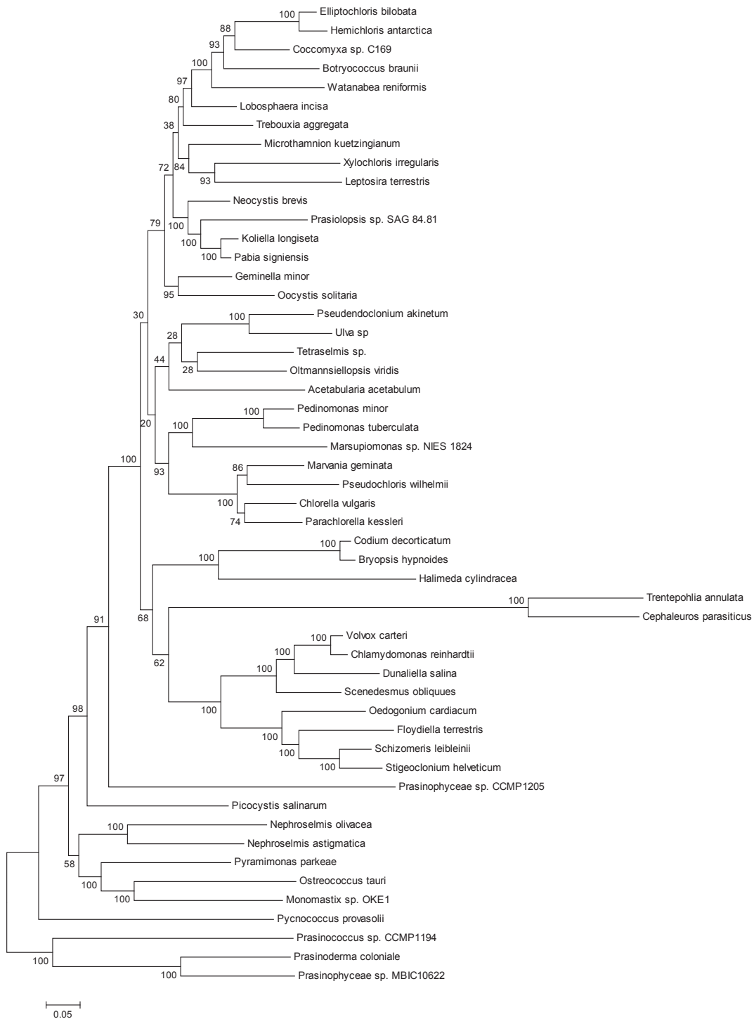
S8 Fig. ML tree with bootstrap values based on AA alignment of 51 chlorophyte genes.
