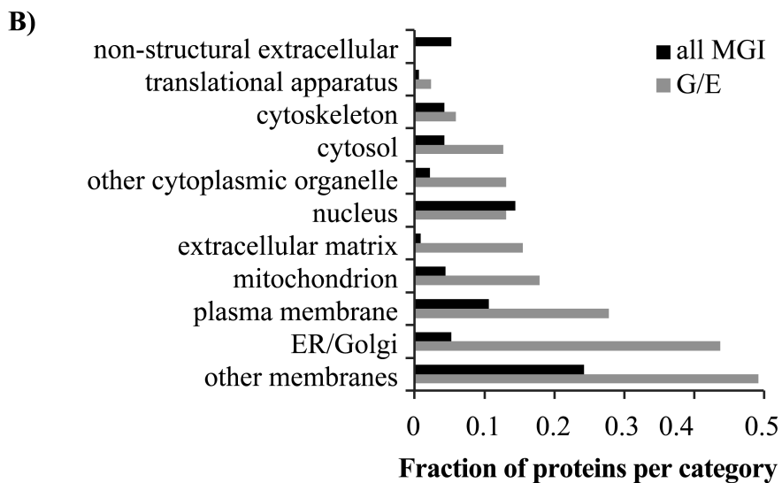
Fig. 1 : Proteins enrichment analysis : A comparative analysis of protein enrichment of the G/E fraction with respect to the total mouse proteome points out a strong enrichment of proteins involved in transport activity (4 times more than in the total mouse) (Pannel A), ER/Golgi proteins are the mostly represented in the G/E fraction (8.3 times more than in the total mouse proteome) (Pannel B).
