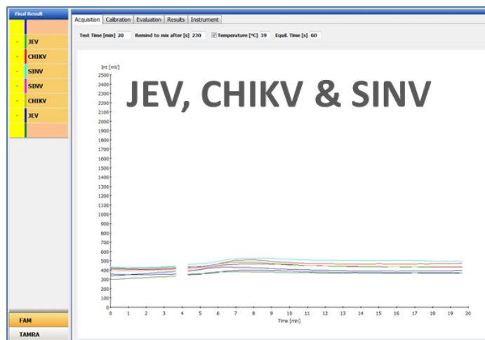
FIG S4. RT-RPA amplification curves of all four DENV serotypes at different dilutions (1000, 100, 50, and 10 RNA copies) (A-D) and other arboviruses (JEV, CHIKV and SINV) (E).
