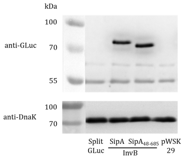
S1 Figure. Western-Blot detecting Gluc fusion proteins in bacterial lysates. Samples were subjected to protein electrophoresis using Bis-Tris gradient gels. A polyclonal anti-Gluc antibody was used to detect SipA 1-685 -C-Gluc 106 and SipA 48-685 -C-Gluc 106 . InvB-N-Gluc 105 could not be detected by this antibody (upper panel). As control DnaK was detected with a monoclonal antibody (lower panel).
