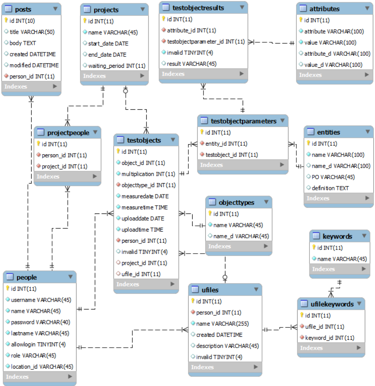
Figure S2. Entity-relationship diagram of the result database
