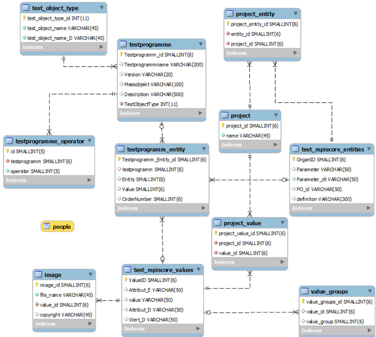
Figure S1. Entity-relationship diagram of the scheme database
