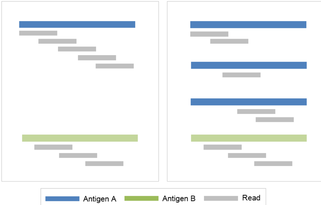
Figure S1. The reads dilution effect. When multiple alleles of Antigen A are archived in the database instead of only one, those alleles compete for reads, leading to the highest amount of reads mapped to an Antigen A allele decreases from 5 to 2, fewer than the 3 mapped to Antigen B.
