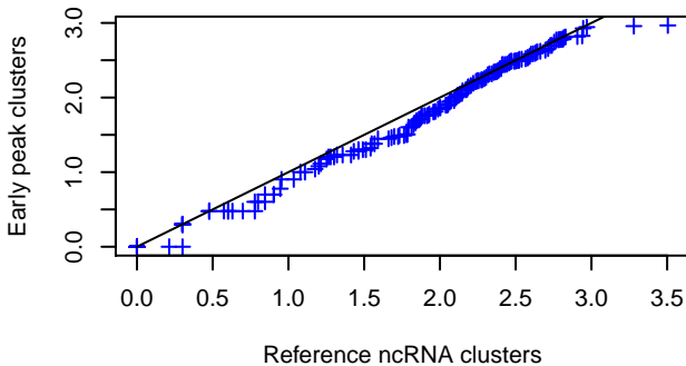
QQ plot log10 DNaseI
