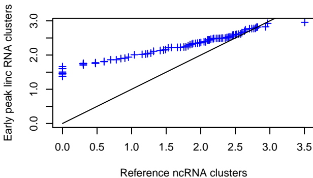
QQ plot log10 DNaseI
