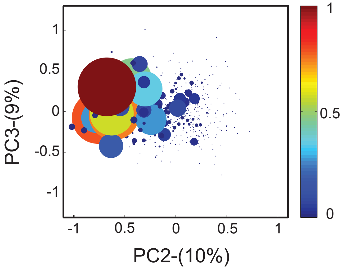
S4 Figure. Results from Principle Component Analysis of the rate constants and its effect on the glioblastoma growth in the LN229 glioblastoma cell line. PC2 is the second principle component and PC3 is the third principle component. Both components contributed about 10% and 9% each to the overall correlation respectively.
