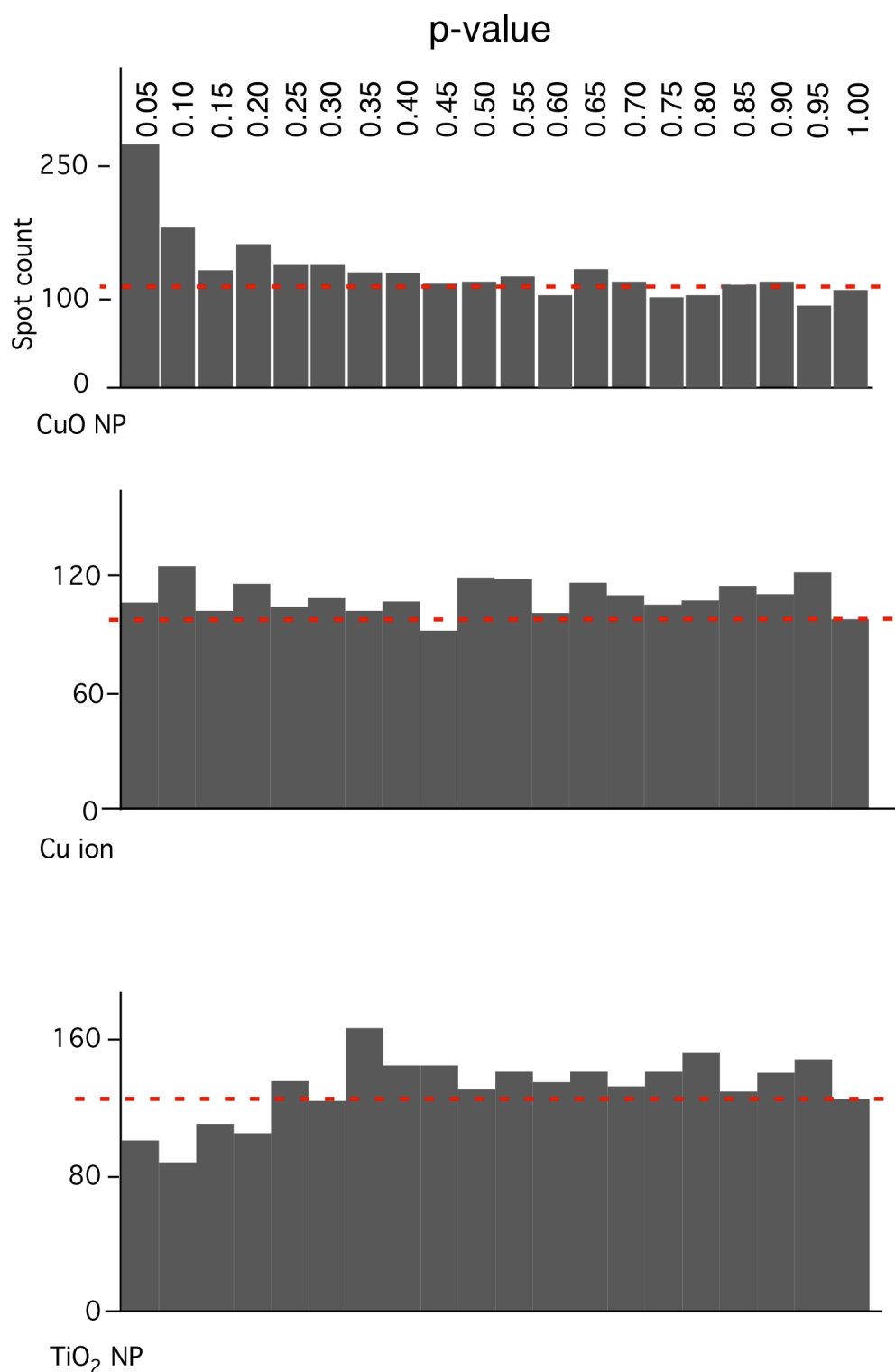
Supporting information Figure S4: Statistical evaluation of the proteomic screen
