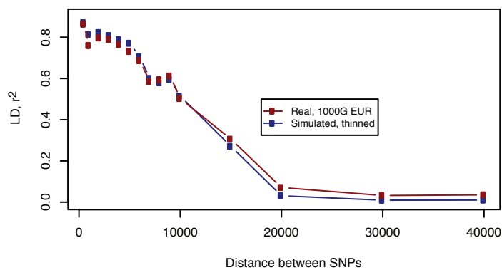
Mean pairwise LD plot for the GATA3 region, 30%<MAF<50%
