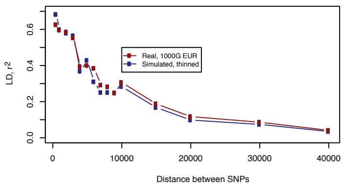
Mean pairwise LD plot for the GATA3 region, 10%<MAF<30%
