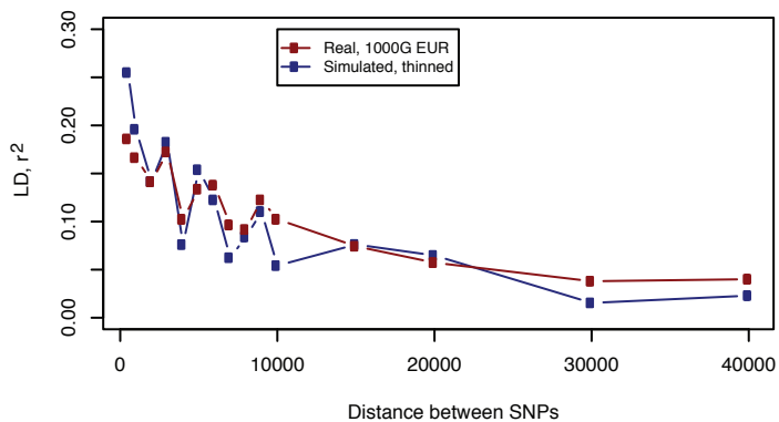
Mean pairwise LD plot for the GATA3 region, 0.5%<MAF<5%
