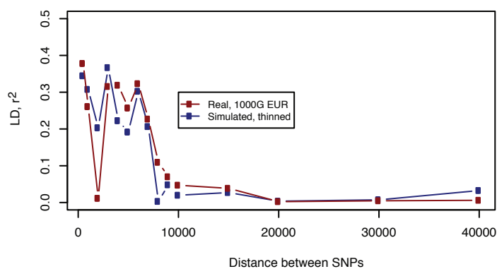
Mean pairwise LD plot for the GATA3 region, 5%<MAF<10%
