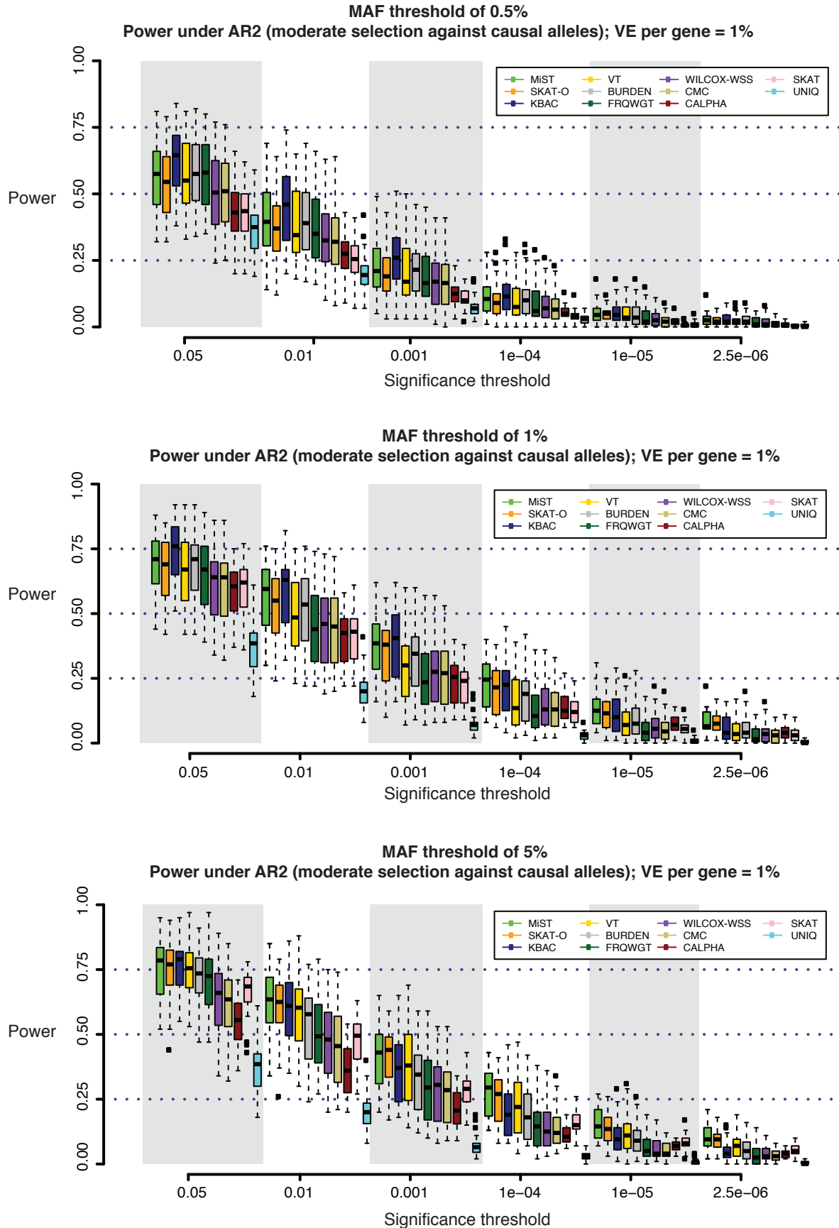
S8 Figure: Power of gene-based methods in 3K samples using different minor allele frequency thresholds for burden testing.
