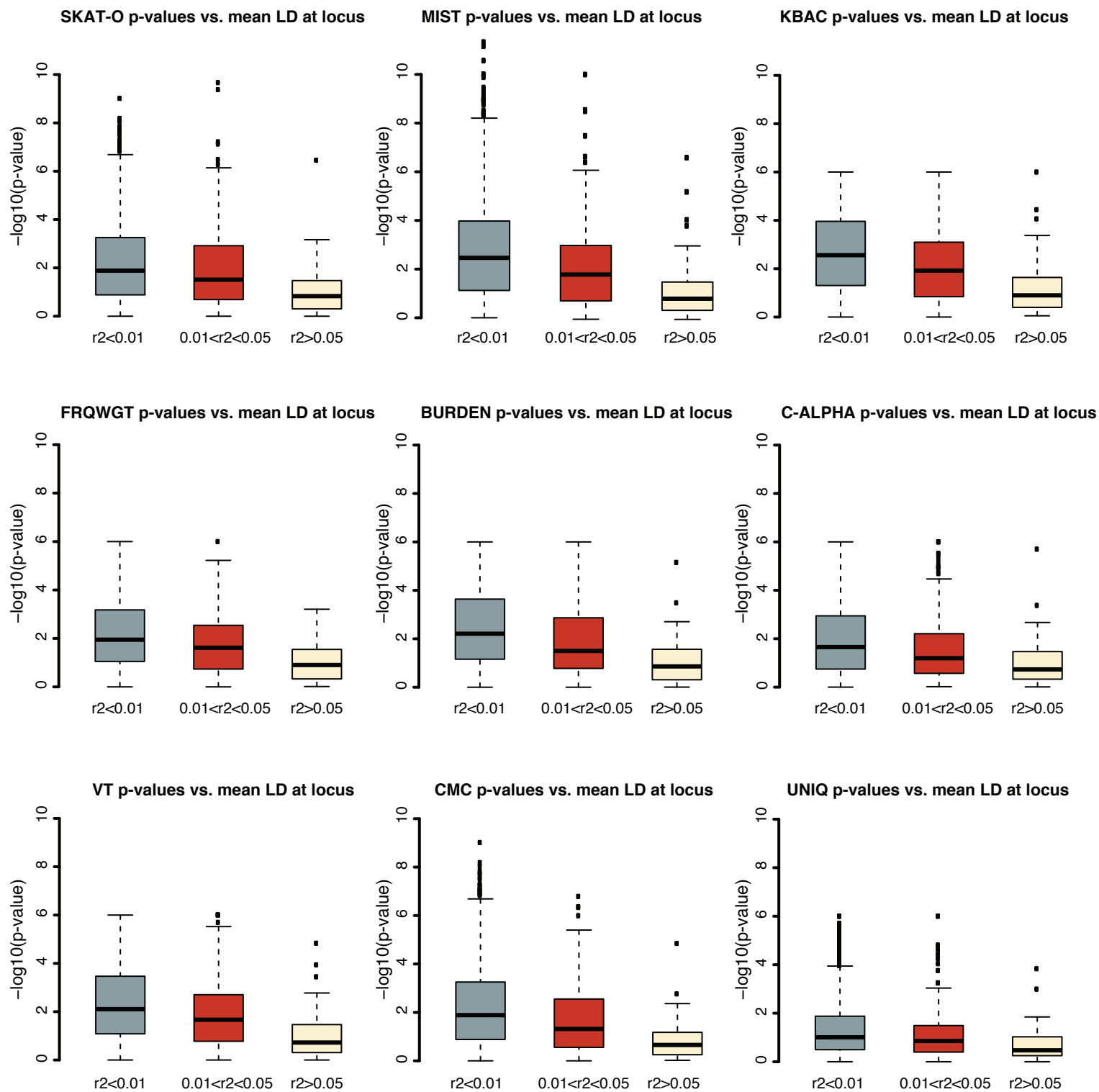
S9 Figure: Effect of linkage disequilibrium between causal variants on power of gene-based tests.
