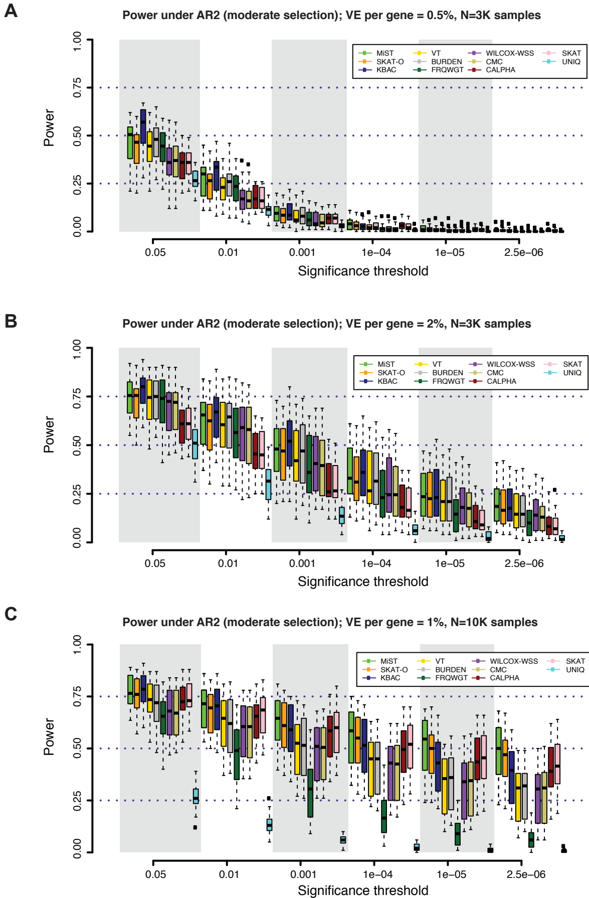
S11 Figure: Power of gene-based tests as a function of locus effect size and sample size.
