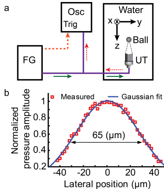
Supplementary Figure S3: Focus calibration of the 50 MHz ultrasonic transducer. a. Experimental setup for ultrasonic transducer calibration. A function generator (FG; DG4162, Rigol, USA) generates a burst including 10 cycles of 50 MHz sine waves, with a peak-to-peak amplitude of 5 V. The burst is sent to the ultrasonic transducer (UT), which emits an acoustic burst correspondingly. The acoustic wave is reflected by the metal ball, and received by the transducer. The echoed signal is digitized using an oscilloscope (Osc; TDS 5034, Tektronix, USA). The peak-to-peak value is proportional to the acoustic pressure amplitude at each position. In the experiment, the transducer is moved along the z direction first to determine the axial focal plane, and then scanned along the y direction to characterize the lateral profile at the focal plane. b. Calibrated acoustic sensitivity at the transducer focal plane, with a FWHM of 65 \mu\text{m} . The red squares are measured data, and the blue curve is a Gaussian fit. The acoustic focal profiles shown in Figure 5 are based on the interpolation of the measured data.
