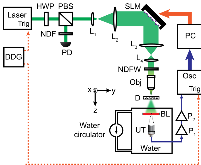
Supplementary Figure S1: Detailed diagram of the experimental PAWS setup. BL, blood layer; D, ground glass diffuser; DDG, digital delay generator; HWP, half-wave plate; L 1-4 , lenses; NDF, neutral density filter; NDFW, neutral density filter wheel; Obj, microscopic objective (10×, 0.25 NA); Osc, oscilloscope; P 1-2 , signal amplifiers; PBS, polarizing beam splitter; PC, computer; PD, photodiode; SLM, spatial light modulator; Trig, trigger signal; UT, ultrasonic transducer; x-y-z, coordinate system.
