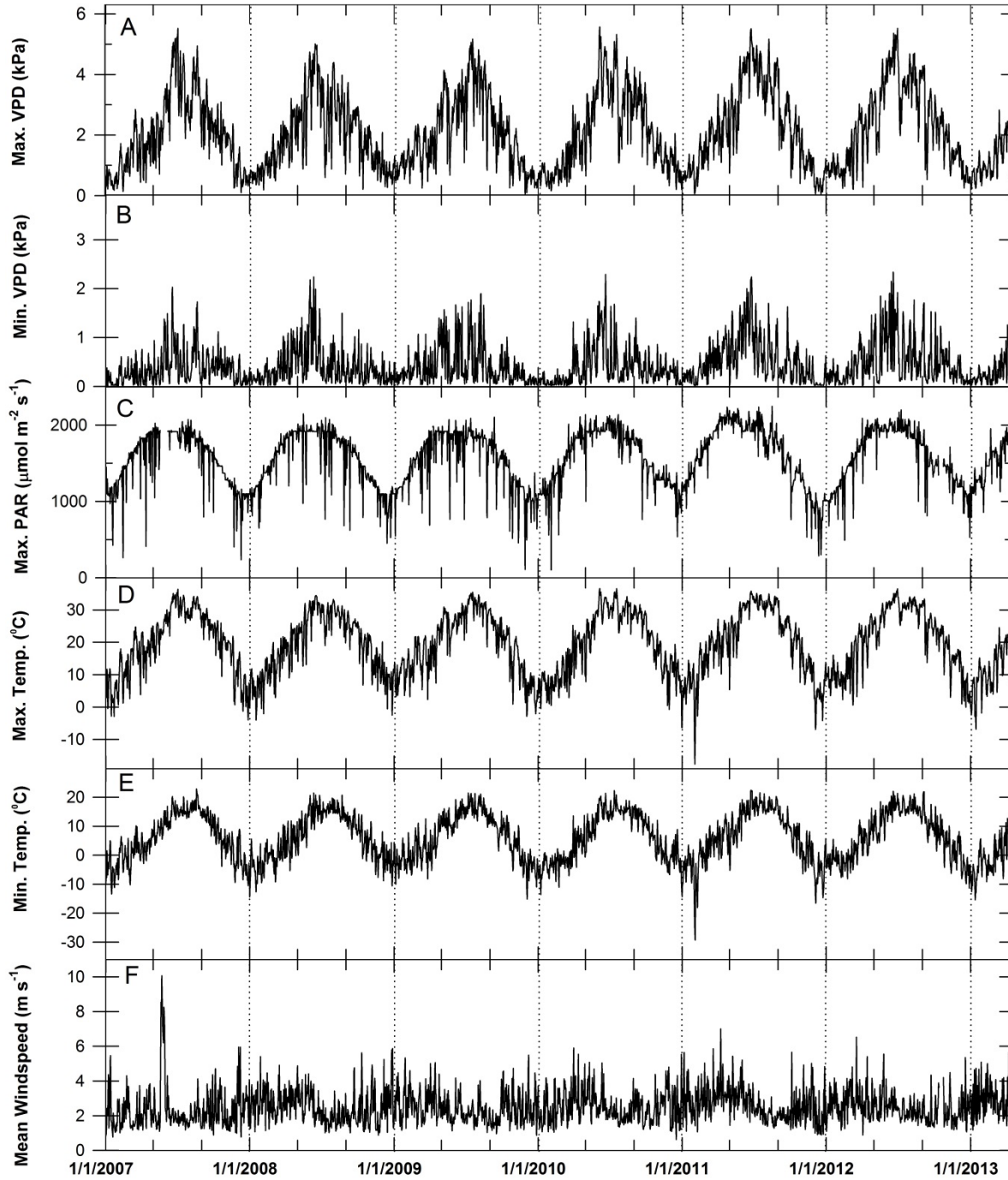
Supplemental - Figure S6. Supplemental climate summary for the 5+ yr period starting in 2007. A) Daily maximum VPD across 5+ yr period, B) Daily minimum VPD , C) Daily maximum PAR , D) Daily maximum temperature, E) Daily minimum temperature, and F) Daily mean wind speed.
