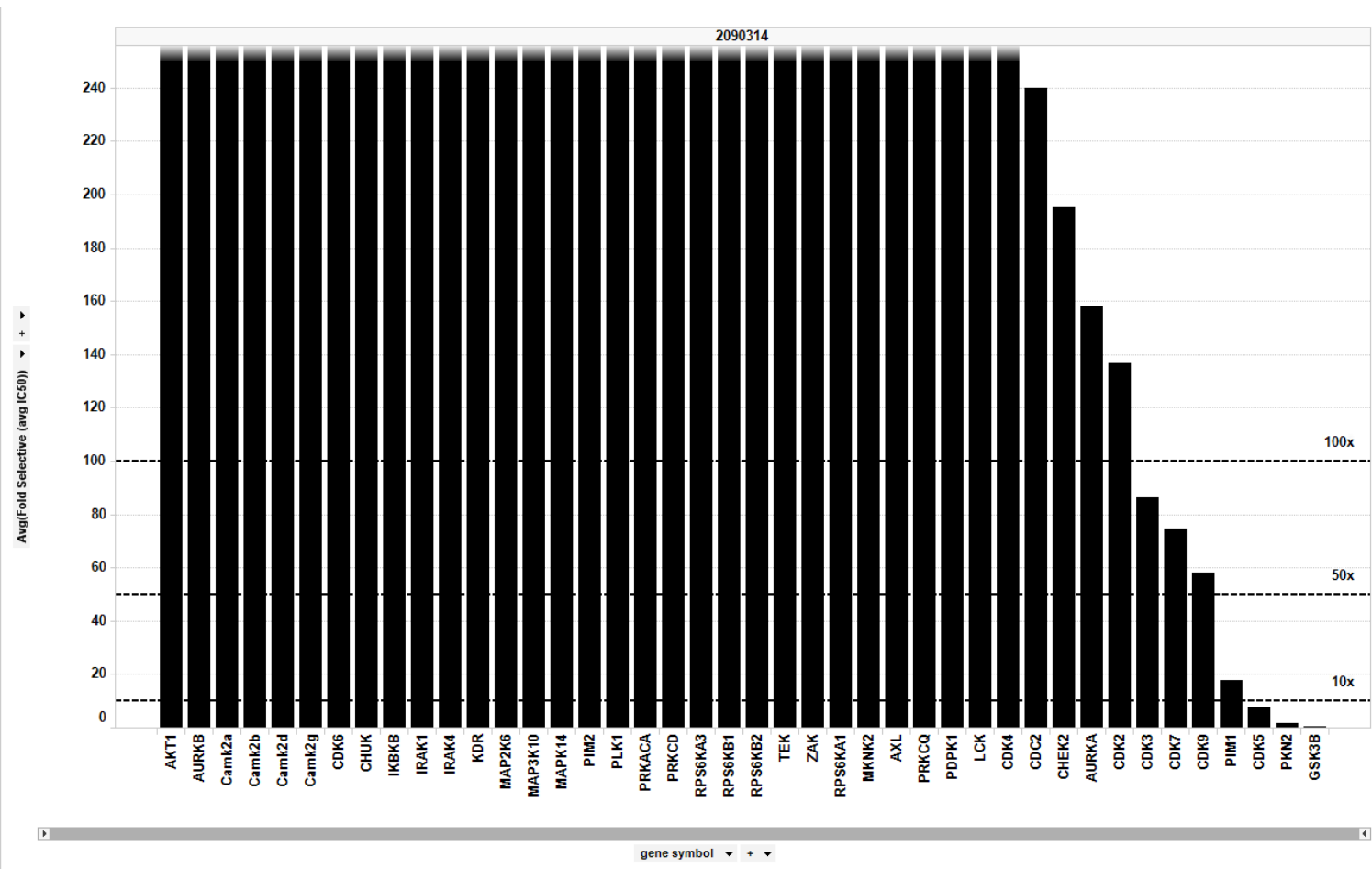
Figure S1. LY2090314 selectivity profile. Single point (20uM) percentage inhibition studies were performed for 200 kinases and IC50 experiments conducted for 44 enzymes. Fold selectivity relative to GSK3 \beta is represented in the figure.
