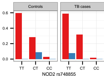
Model 8 dominant-dominant
