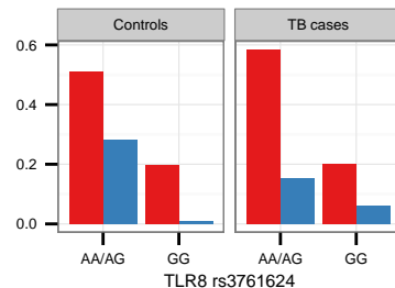
Model 16 recessive-dominant
