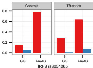
Model 17 recessive-dominant
