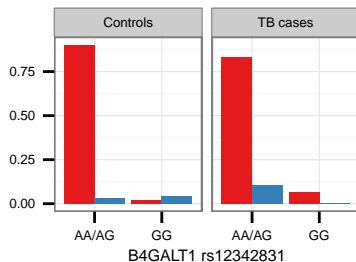
Model 9 dominant-additive
