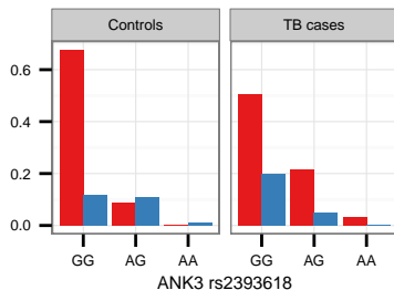
Model 18 recessive-additive
