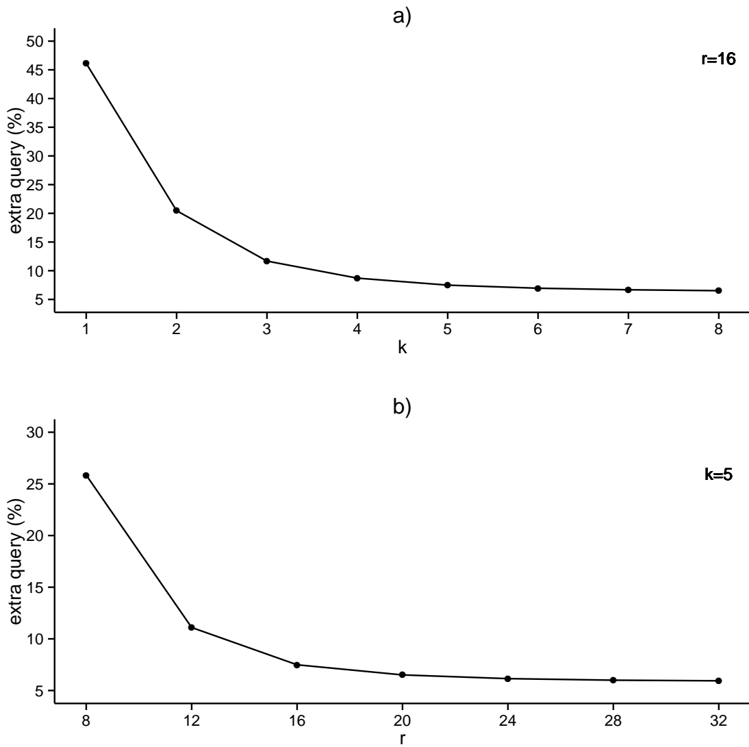
Supplementary Figure 1. Extra dispatched reads vs. r and k . (a) Percentage of extra dispatched reads vs. the number of hash functions, k , for the fixed value of r = 16 on C. elegans dataset. (b) Percentage of extra dispatched reads vs. the number of bits per item, r , for the fixed value of k = 5 on C. elegans dataset.
