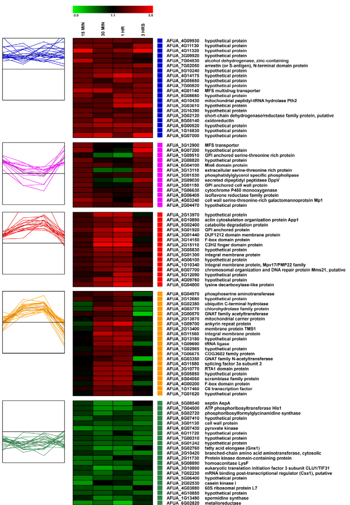
Supplemental Figure 2: K-means clustering of gene expression profiles of genes significantly ( p < 0.05 ) differentially expressed in A. fumigatus at least at two time points after exposure to platelets.
