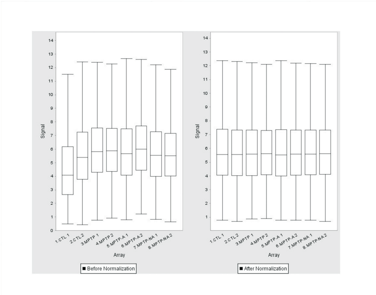
Figure S1 - Box plot before and after normalization.
