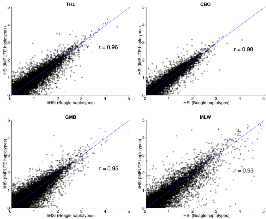
S. Figure 3. Pearson's correlation ( r ) between |iHS| metrics calculated from Beagle- or IMPUTE-imputed genotypes. Diagonal line indicates line of equality.
