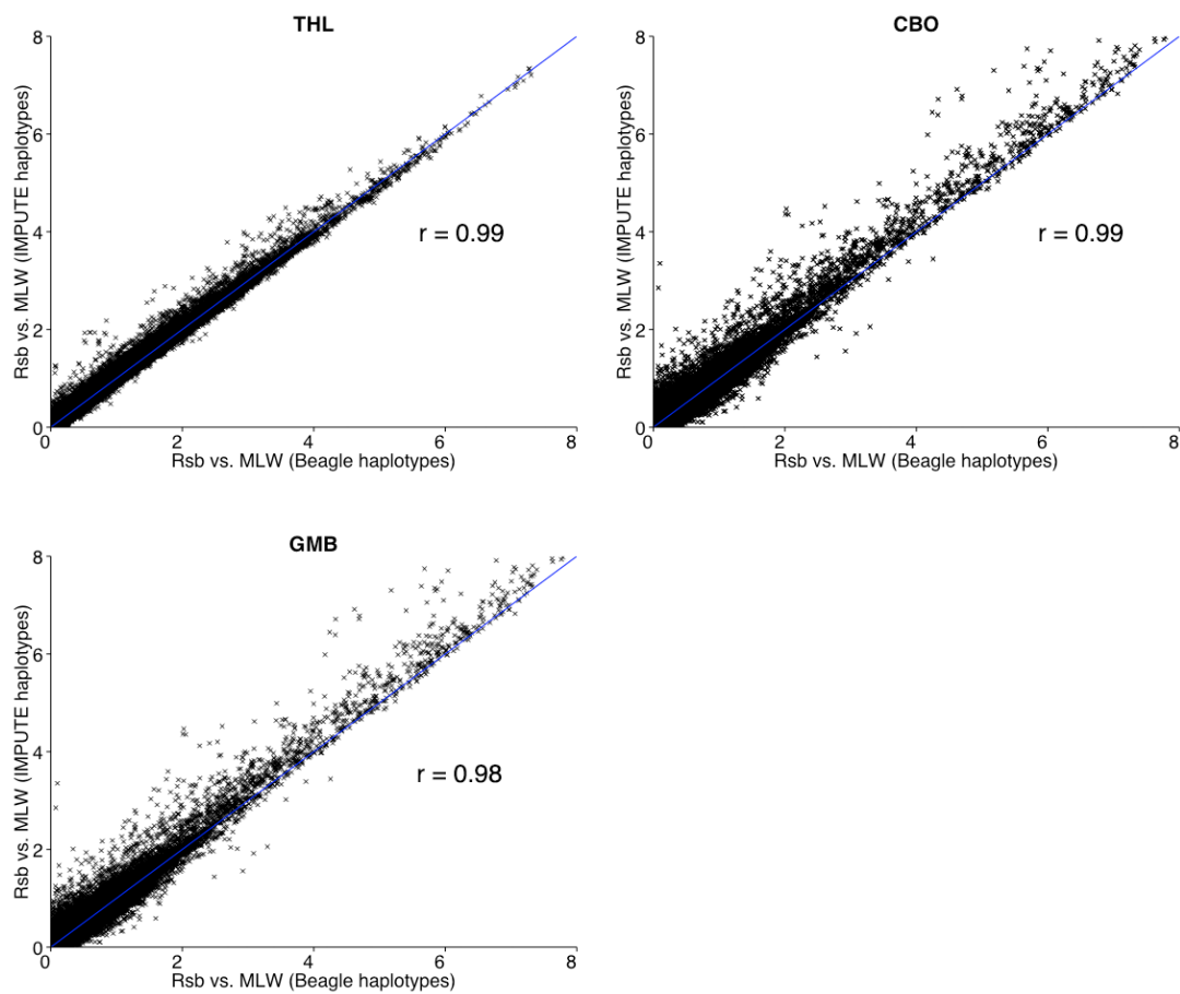
S. Figure 4. Pearson's correlation ( r ) between Rsb metrics calculated from Beagle- or IMPUTE-imputed haplotypes. Malawi is used as the reference population. Diagonal line indicates line of equality. Mass of points above the line indicates that IMPUTE-derived haplotypes systematically produce larger Rsb values than Beagle-derived haplotypes.
