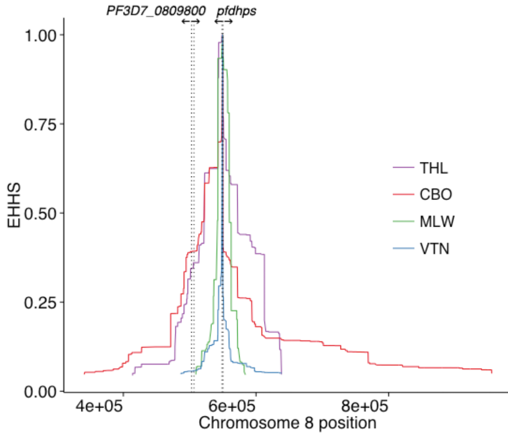
S. Figure 8. Analysis of site-specific EHH around a core SNP within dhps . With Malawi as the reference population, Rsb metrics in Thai and Cambodian populations indicate no signal for positive selection in dhps but do indicate a strong signal for positive selection in neighbouring PF3D7_0809800 . In contrast, dhps is detected by using Vietnam (VTN) as the reference population.
