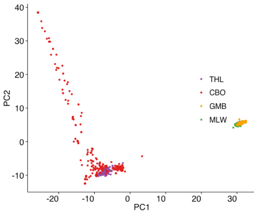
S. Figure 9. Principal components analysis of P. falciparum isolates using unimputed (top) and Beagle-imputed (bottom) SNP data. PC1 and PC2 refer to the first and second principal components, respectively.
