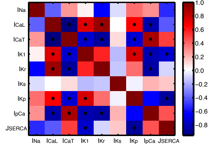
Combined protocol
