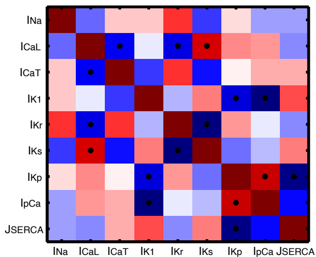
Single AP
