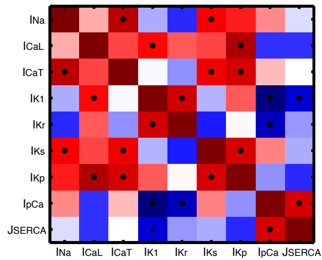
Stochastic pacing
