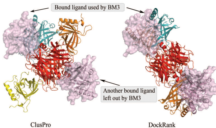
Figure S7. The top 5 conformations ranked by DockRank and ClusPro for docking case 1RLB. Both ligands of the bound complex downloaded from PDB are shown in pink surface representation. Figure generated using PYMOL [70].
