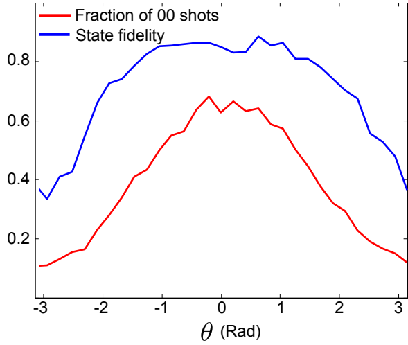
Supplementary Figure 1. Fidelity and Error Angle. a. Fidelity and fraction of down-down shots as a function of bit error angle.
