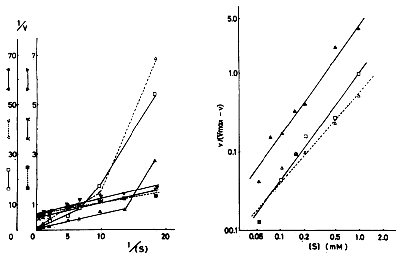
Figure 3. Kinetics of the BCKDH complex in disrupted lymphoblastoid cell lines from MSUD subjects. The incubation and protein added were the same as for Fig. 1. The cell lines were the same as for Fig. 2. (a) Lineweaver-Burk plots of the BCKDH complex activities in the cell lines; K.F. ( \times ), R.F. ( \blacksquare ), K.Y. ( \Delta ), Y.T. ( \blacktriangle ), GM 1655 ( \square ) and GM 1366 ( \blacktriangledown ). (b) Hill plots of the BCKDH activities in the cell lines; K.Y. ( \Delta ), Y.T. ( \blacktriangle ) and GM 1655 ( \square ).
