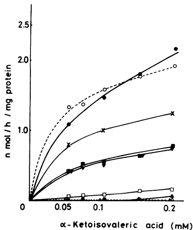
Figure 4. Kinetics of the E_1 component activity in disrupted lymphoblastoid cell lines from disease-free and MSUD subjects. Radiochemical ferricyanide assays were carried out as described in Methods in the presence of 0.2 mM-TPP with \alpha -keto-[1- ^{14} C]-isovaleric acid as the variable substrate. The disrupted-cell suspensions used were the same as for Fig. 1. The cell lines from MSUD subjects are the same as
