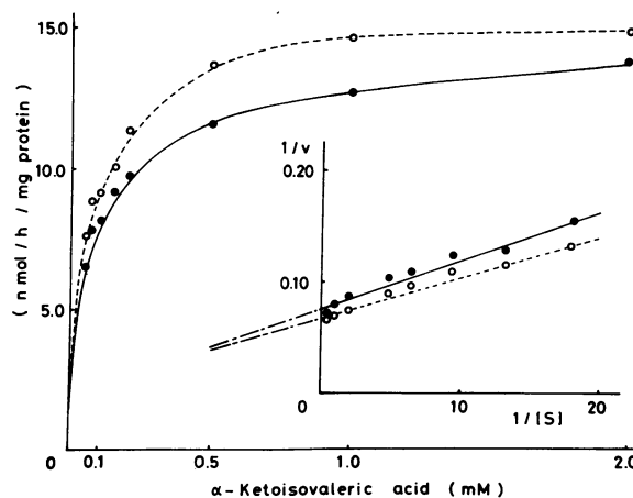
Figure 1. Activities of BCKDH complex in disrupted lymphoblastoid cell lines from disease-free Japanese. The rate of the overall reaction catalyzed by the multienzyme complex was measured in the presence of cofactors, as described in Methods, with \alpha -keto [ 1\text{-}^{14}\text{C} ]isovaleric acid as the variable substrate. Disrupted cell suspensions (equivalent to 0.8–1.0 mg of protein) were used as the enzyme source. All kinetic data were determined under conditions with which a linear relationship with time and the amount of protein added observed. Lineweaver-Burk plots are shown in the insert. \circ , control 1; \bullet , control 2.
