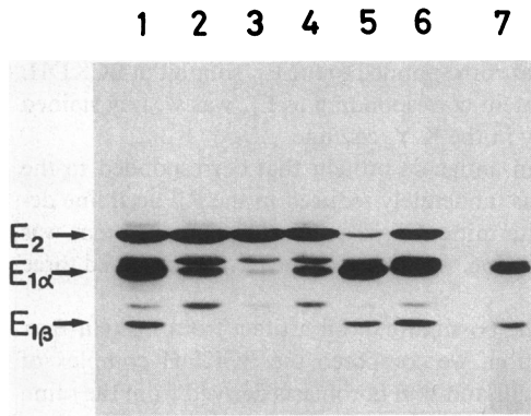
Figure 6. Immunoblots of the BCKDH complex in lymphoblastoid cell lines from MSUD subjects. Mitochondrial extracts containing 120 \mu g protein each were resolved by SDS-PAGE. The BCKDH peptides were identified by immunoblotting, as described under Methods. The BCKDH ( E_1 + E_2 ) complex peptides were the same as for Fig. 5. (Lane 1) A disease-free cell line; (lanes 2-4) GM 1655 and cell lines from classical type MSUD patients (K.Y. and Y.T.); (lanes 5-6) cell lines from intermittent type MSUD patients (R.F. and K.F.); (lane 7) GM 1366. The blot was intentionally overexposed to a chromogenic substrate to demonstrate absence of the E_{1\beta} subunit protein, except for lane 7. These experiments were repeated twice using different preparations with essentially identical results.
