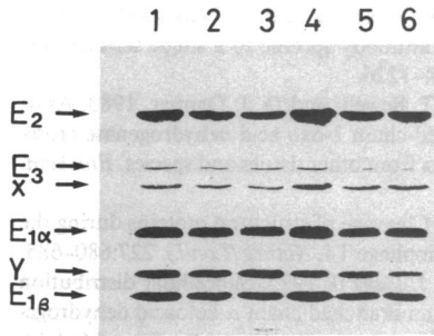
Figure 8. Immunoblots of the PDH complex in lymphoblastoid cell lines from MSUD subjects. The procedures were the same as for Fig. 6 except that antiserum raised against the bovine PDH complex was used for the immunoblotting. The cell lines used were the same as for Fig. 6,
