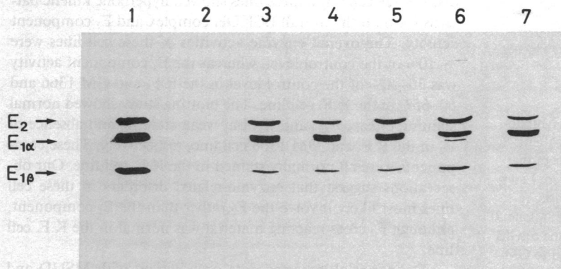
Figure 5. Immunoblots of the BCKDH complex. Various protein samples were resolved by SDS-PAGE and then transferred electrophoretically onto nitrocellulose paper, as described in Methods. BCKDH immunoreactive proteins were detected by the protein blot technique, using affinity purified antibody. The BCKDH ( E_1 + E_2 ) complex peptides were, in decreasing size: ( E_2 ) dihydrolipoyl transacetylase ( M_r 52,000), ( E_{1\alpha} ) the \alpha -subunit of branched-chain \alpha -keto acid decarboxylase ( M_r 46,000), and ( E_{1\beta} ) the \beta -subunit of branched-chain \alpha -keto acid decarboxylase ( M_r 37,000). (Lane 1) The purified bovine kidney BCKDH complex (0.5 \mu g) with its component peptides, as indicated; (lane 2) the purified bovine heart PDH complex (3.3 \mu g); (lanes 3-5) mitochondrial extracts (120 \mu g) from disease-free lymphoblastoid cell lines; (lanes 6 and 7) mitochondrial extracts of human liver and kidney, respectively (120 \mu g of each protein).
