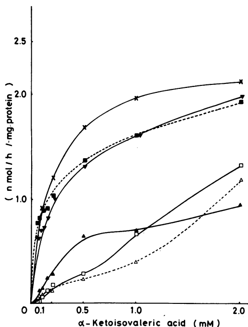
Figure 2. Activities of BCKDH complex in disrupted lymphoblastoid cell lines from MSUD subjects. The incubation and protein added were the same as for Fig. 1. GM 1655 ( \square ) and GM 1366 ( \blacktriangledown ) are MSUD cell lines obtained from the Human Mutant Cell Repository, Camden, NJ. K.Y. ( \Delta ) and Y.T. ( \blacktriangle ) are cell lines from classical type MSUD patients. R.F. ( \blacksquare ) and K.F. ( \times ) are cell lines from intermittent type MSUD patients.
