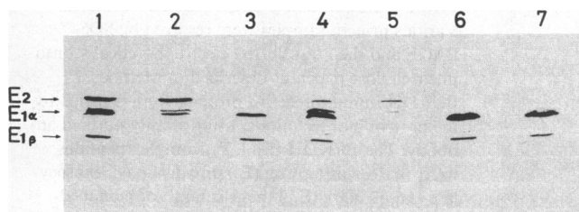
Figure 7. Comparison of the BCKDH ( E_1 + E_2 ) complex in lymphoblastoid cells and in skin fibroblasts derived from the same patients with MSUD. The procedures were the same as for Fig. 6 except that skin fibroblast extracts containing 250 \mu g protein were applied. Lanes 1-3 and lanes 4-7 are lymphoblastoid cells and skin fibroblasts, respectively. (Lane 1) A disease-free cell line; (lane 2) GM 1655; (lane 3) GM 1366; (lane 4) a disease-free cell; (lane 5) GM 1654; (lane 6) GM 1364; (lane 7) GM 612. GM 1655 and GM 1366 correspond to GM 1654 and GM 1364, respectively. A lymphoblastoid cell line corresponding to GM 612 was not available.
