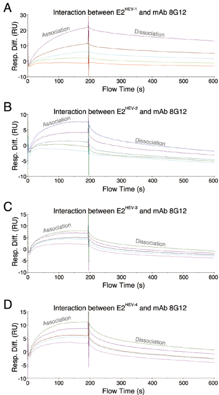
Supplementary information, Figure S1 E2 and mAb 8G12 binding curves in Surface Plasma Resonance (SPR). Total 5 concentrations of E2 in serial dilution were injected to mAb 8G12-bound chip. These binding curves were used to calculate the affinity constants. The experiments were repeated twice and the results are consistent.
