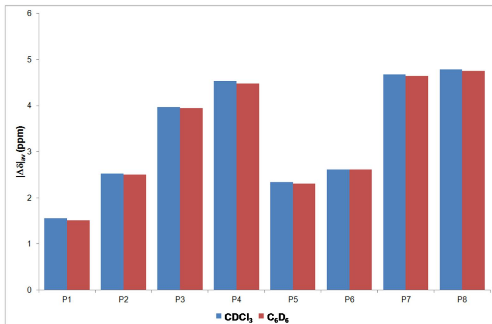
Dataset S3. Mean absolute deviation plot of experimental and calculated 13 C chemical shifts for Cucumene in CDCl 3 and C 6 D 6 .
