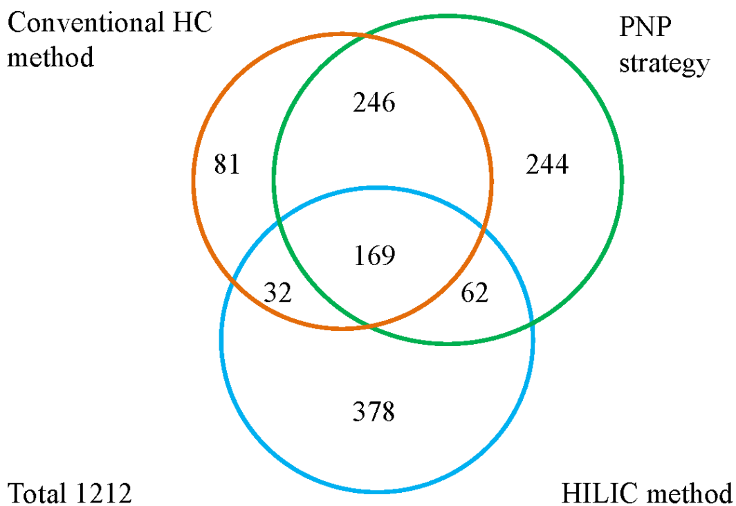
Figure S6 | Performance of the PNP strategy. Comparison of the overlaps of glycosites identifications for conventional HC method, PNP strategy and the HILIC method.
