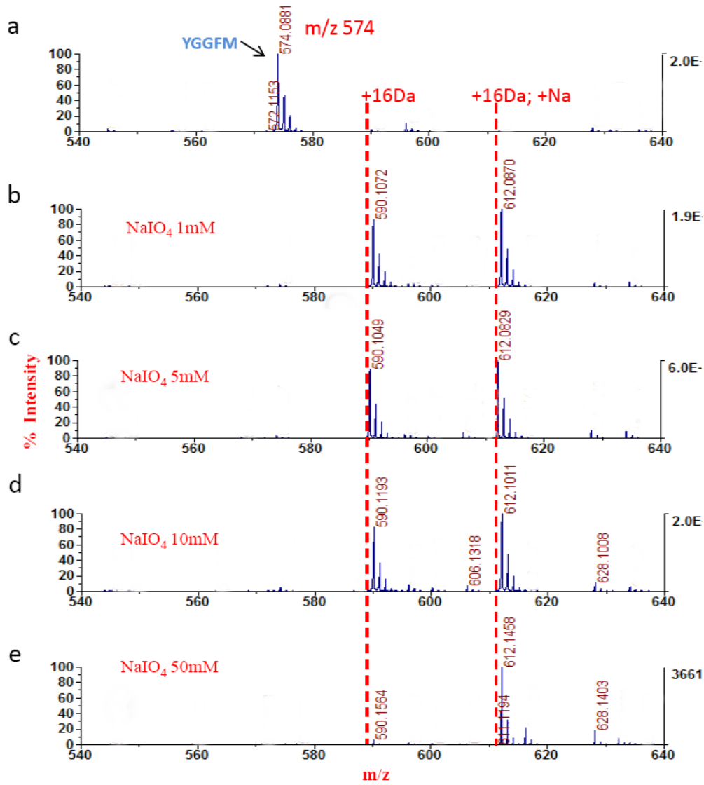
Figure S2 | The side reactions on Met. (a-e) MALDI mass spectra of the Met containing peptides YGGFM (0.01 \mu\text{g}/\mu\text{L} , 0.5 \mu\text{L} ) oxidized at 0, 1, 5, 10, 50 mM \text{NaIO}_4 .
