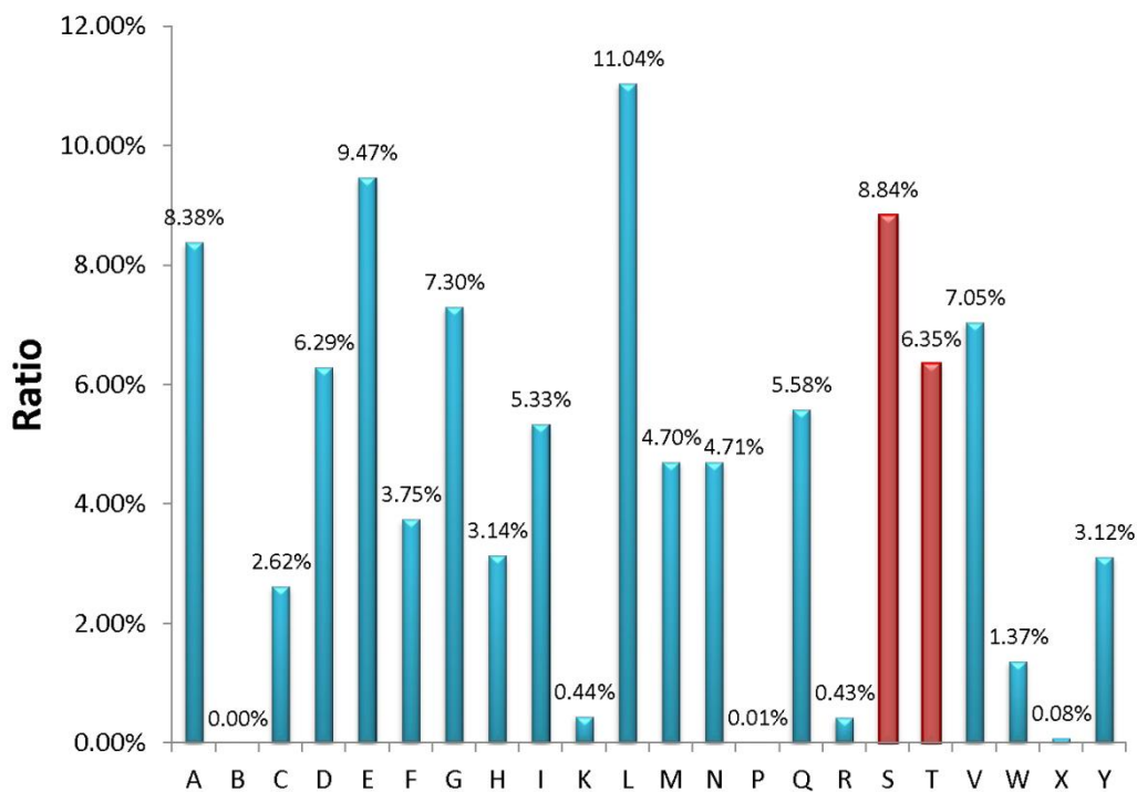
Figure S4 | The N-terminal amino acid residue distribution of in silico tryptic peptides of mouse proteome (database: IPI mouse v3.87).
