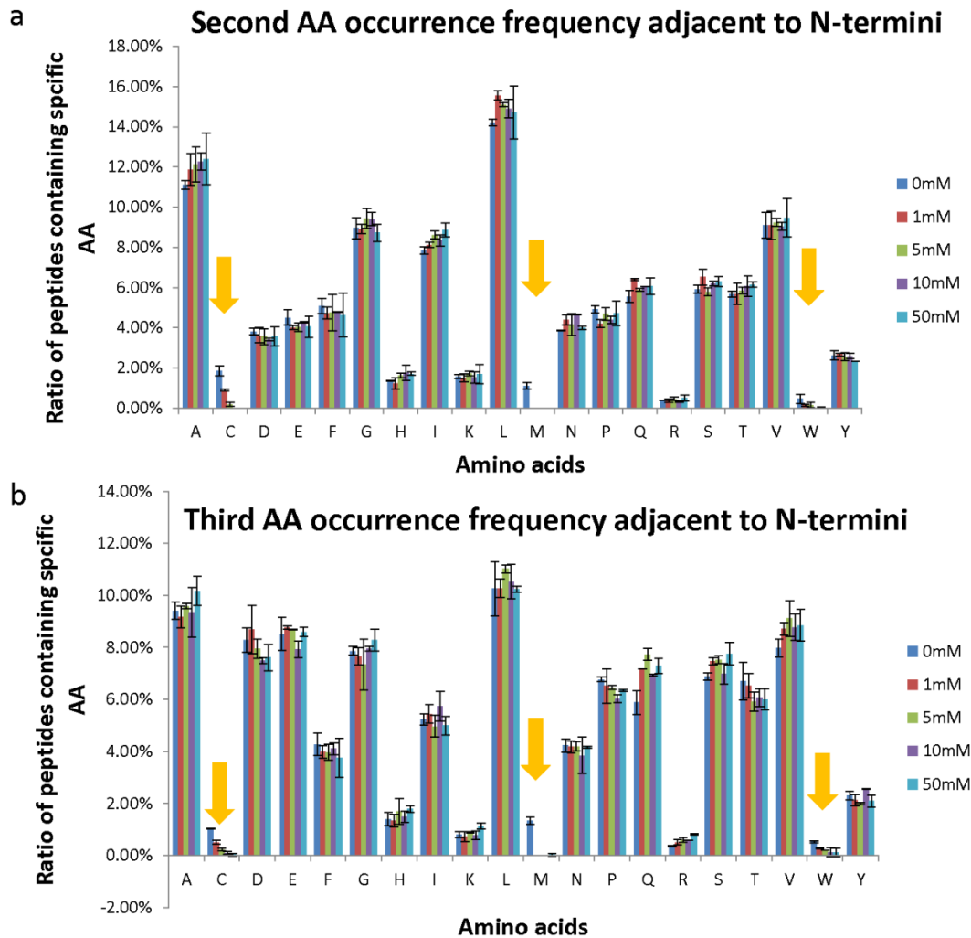
Figure S1 |Proteome-wide amino acid frequency check approach to locate the possible side reaction sites. (a) The percentage of peptides with the second residue from the N-termini with a specific type of amino acid residue in all peptides. (b) The percentage of peptides with the third residue from the N-termini with a specific type of amino acid residue in all peptides. Above data were averaged from 4 replicate experiments (error bars represent the standard deviation )
