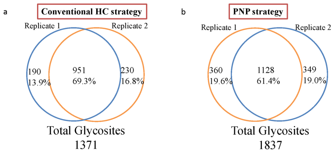
Figure S7 | Comparison of replicate runs. (a) Conventional HC method. (b) PNP strategy.
