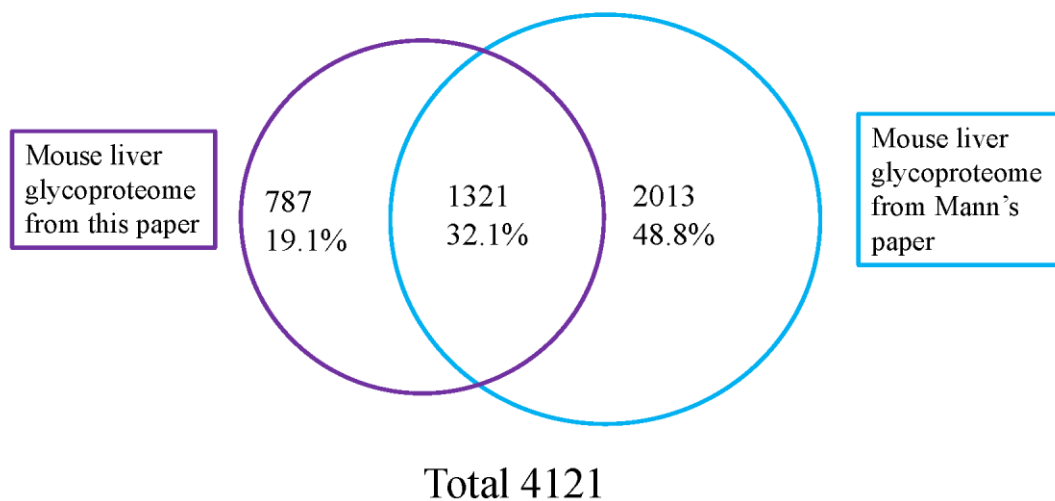
Figure S8 | Comparison of large scale mouse liver glycoproteome dataset acquired in this paper with the dataset acquired from lectin affinity methods reported in literature. Overlap of the glycosites identified in this work and in the work by using lectin affinity methods 1 .
