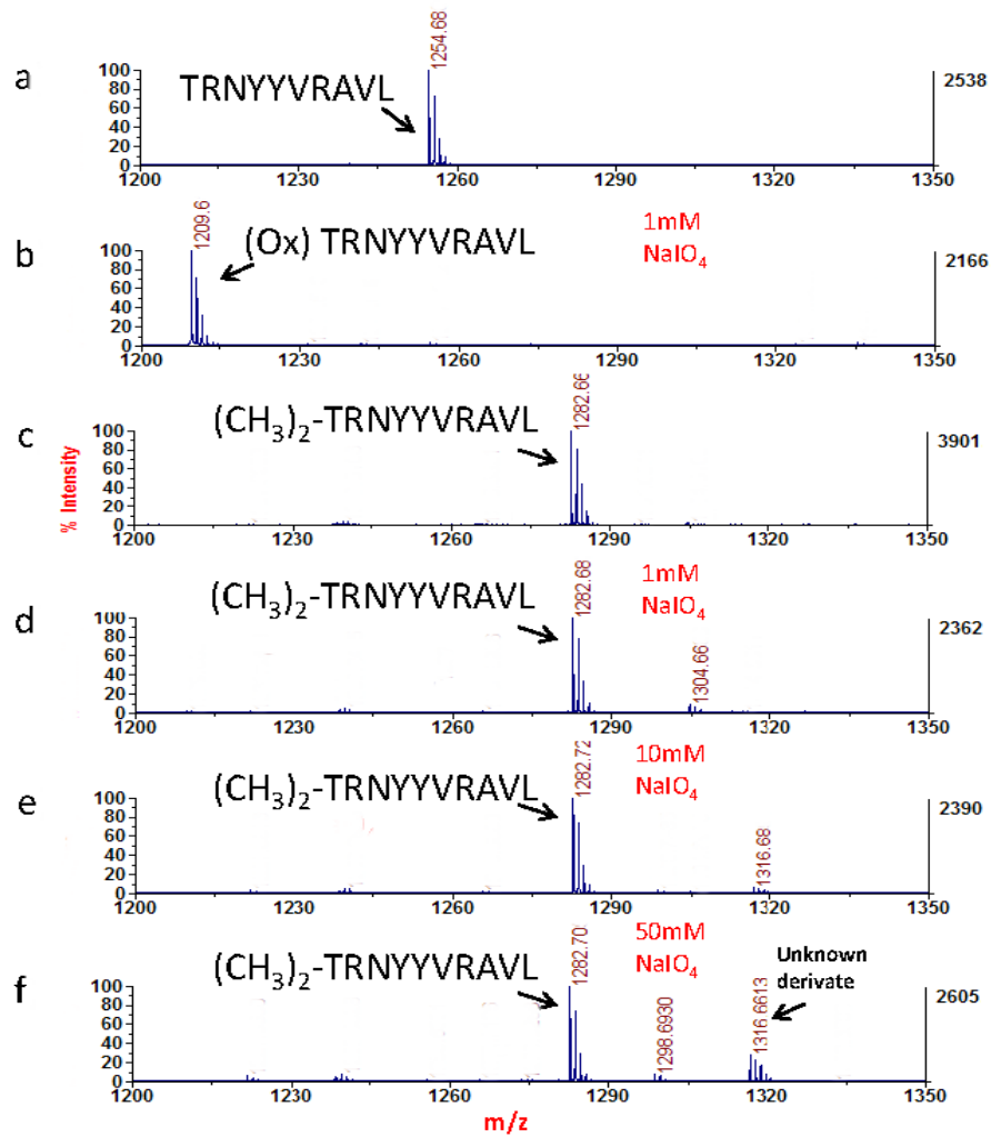
Figure S3 | PNP strategy prevents the oxidation of peptides with N-terminal Thr. MALDI mass spectra of the standard N-terminal Thr peptide TRNYYVRAVL (0.01 \mu\text{g}/\mu\text{L} , 0.5 \mu\text{L} ) with or without dimethyl protection oxidized in periodate solutions with different concentrations: (a) without protection, without oxidation; (b) without protection, with oxidation (1mM \text{NaIO}_4 ); (c) with protection, without oxidation; (d) with protection, with oxidation (1mM \text{NaIO}_4 ); (e) with protection, with oxidation (10mM \text{NaIO}_4 ); (f) with protection, with oxidation (50mM \text{NaIO}_4 ).
