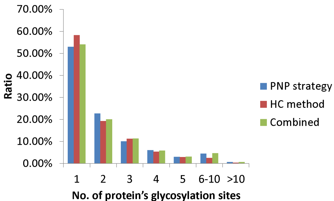
Figure S9 | Distribution of singly and multiply glycosylated proteins. The ratio of identified proteins with multi-glycosites in PNP strategy is higher than the conventional HC method.
