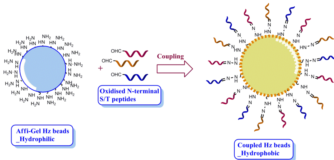
Figure S5 | Surface property change of hydrazide beads during glycopeptide enrichment in the conventional HC method. Enormous peptides with N-terminal Seri/Thr are also coupled onto the hydrazide beads in the conventional HC method because they are also oxidized. This makes the surface of the beads changing from hydrophilic to hydrophobic, from neutral to charged. While in the PNP strategy, the bead surface will not change significantly because these peptides will not be bound.
