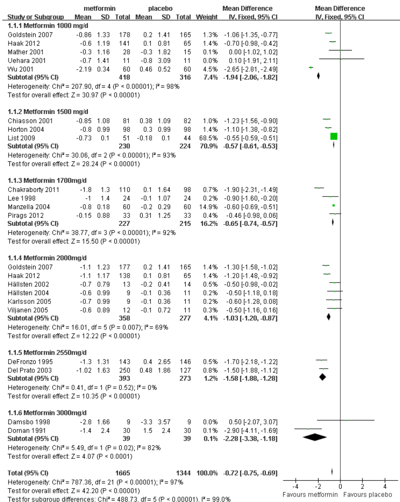
S3 Fig. Sensitivity analysis: Glucose lowering effect (reduction of HbA 1c ) of metformin versus placebo (use a fixed-effect model instead)
